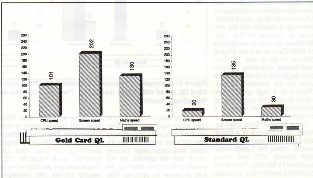
Figure 2: A comparison between a standard QL and a Gold Card QL running DR-DOS 5.0 under Conqueror. The test come from the Checkit benchmarking utility.
